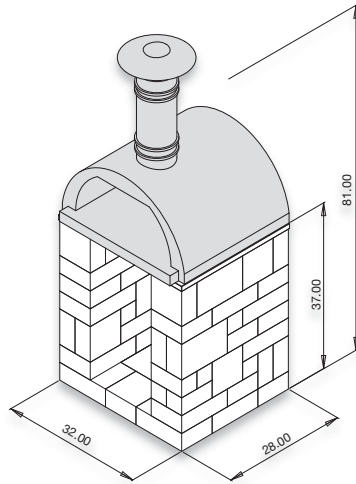
Wood-Fired Outdoor Oven Woodbox/Stand Cabinet
