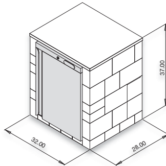
Refrigerator Cabinet (Optional refrigerator)
