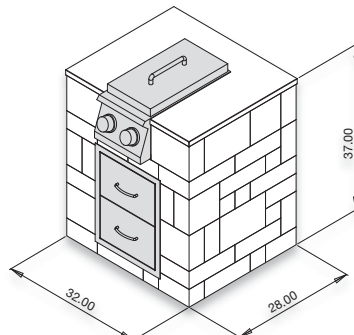
Side Burner Cabinet
